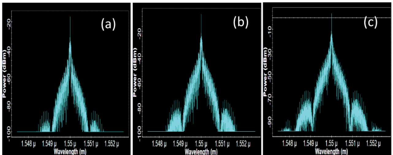
Figure 4 - Optical spectrums at (a), (b), and (c) both after AOF (signal amplified by SPM induced due to variation of input signal power).
