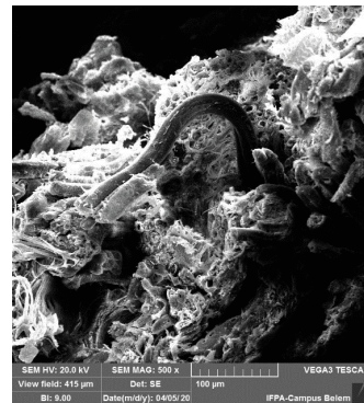
Figure 16 - Fractography of timbó-açu fiber. 500x
