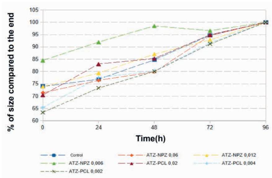
Figure 5: Body growth curves of Daphnia magna fed on algae ( Raphidocelis subcapitata ) previously exposed to ATZ-NPZ (atrazine encapsulated in zein nanoparticles) and ATZ-PCL (atrazine encapsulated in poly-epsilon-caprolactone nanoparticles) in the absence of NOM (humic acid), under different herbicide concentrations (mg/L).
