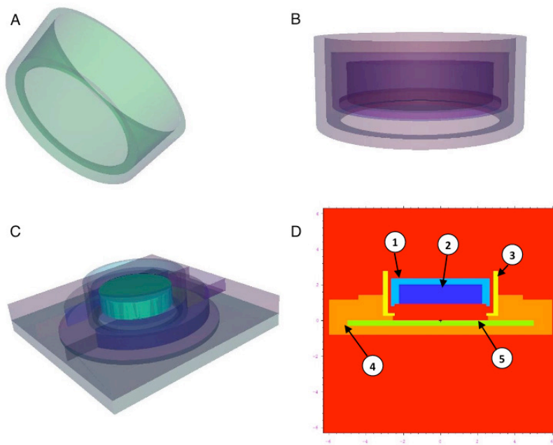
Figure 2: MCNP6 modeling. A) ABS plastic carcass; B) LND Geiger inside ABS carcass; C) Three-dimensional representation of the model with the GM detector in green; D) Vised® image of the model in the YZ plane showing: 1) 440 stainless steel cathode; 2) Sensitive volume (Ne/Cl gas); 3) ABS carcass; 4) Acrylic calibration apparatus; 5) Planar aluminum source.
