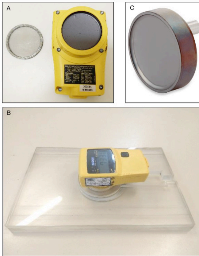
Figure 1: Detector and experimental setup. A) RDS-80A detector with the protective grid removed; B) Acrylic calibration apparatus with planar source; C) Geiger LND Counter – 7313.
