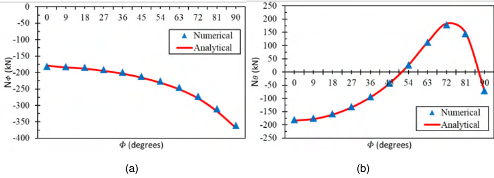
Figure 8 – Comparative graphics for the hinge supported dome: (a) N_\phi (b) N_\theta
