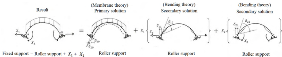
Figure 4 – The force method solution
