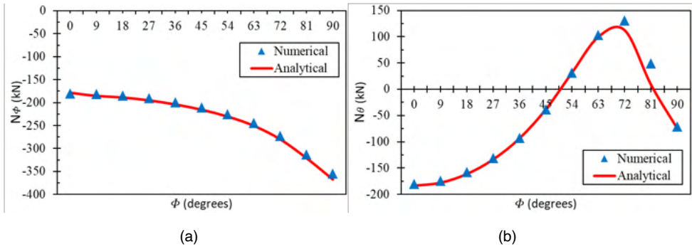
Figure 9 – Comparative graphics for the fixed supported dome: (a) N_\phi (b) N_\theta
