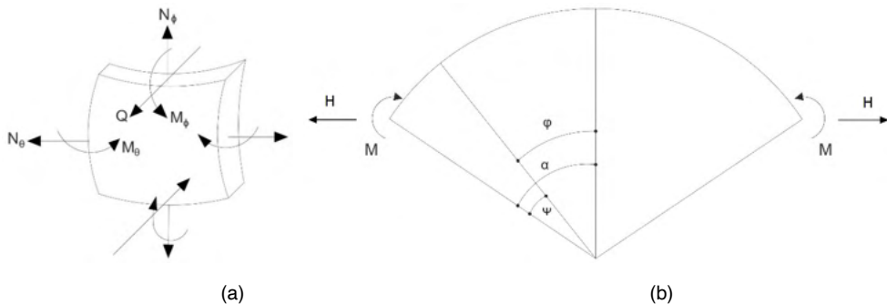
Figure 3 – General shell under load: (a) Designations of differential element (b) Bending moment acting on the edge of the shell
