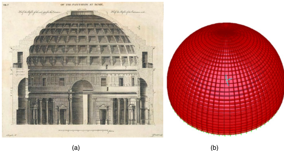
Figure 5 – Analyzing the Pantheon: (a) Drawing of the geometry of the Pantheon: back cross section (b) Mash of the numerical model
