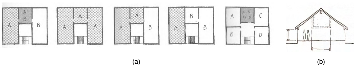
Figure 4: (a) neutral environments for different uses; (b) Usable Attic: adequate ceiling height and structural system.
