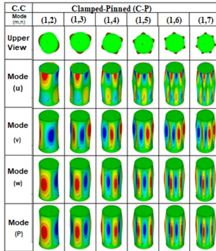
Clamped-Pinned (C-P)
