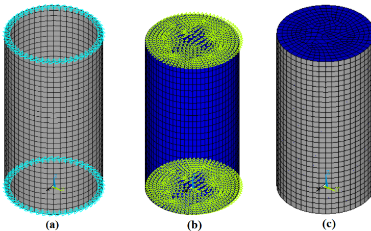
Figure 2: Numerical models: (a) Uncoupled shell; (b) Uncoupled fluid and (c) Fluid-Structure interaction.
