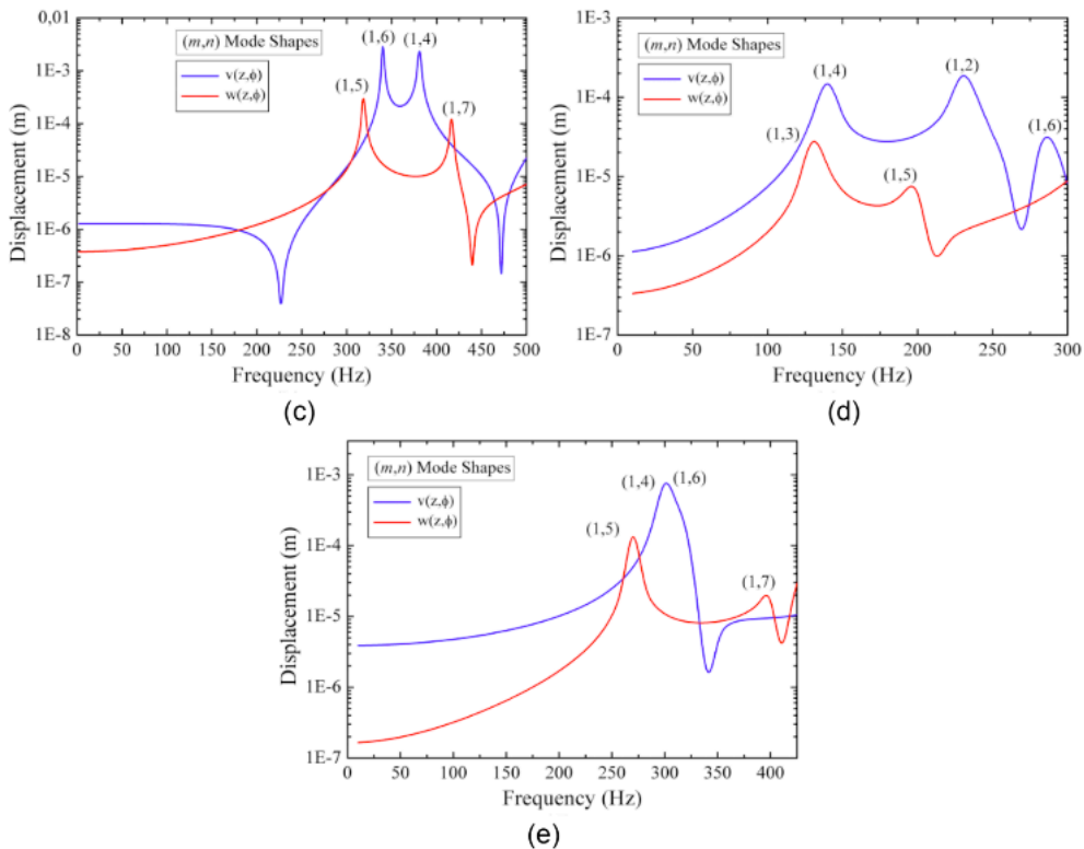
Figure 5: Frequency spectrum for a cylindrical shell uncoupled (empty) for position in z = L / 2 and \phi = 180^\circ : (a) pinned-pinned, (b) pinned-free, (c) clamped-clamped, (d) clamped-free e (e) clamped-pinned.
