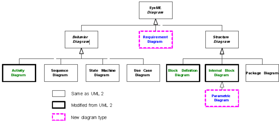
Figure 3 - SysML diagram taxonomy.
