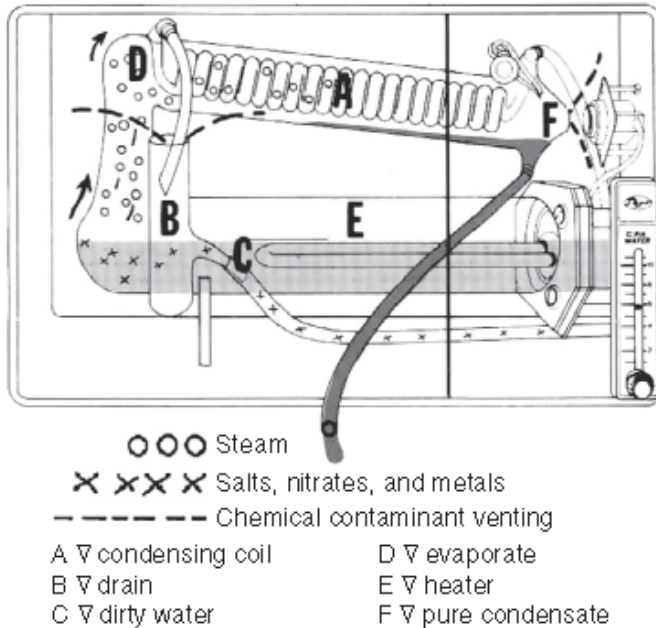
Figure 4. Continuous water distiller.
