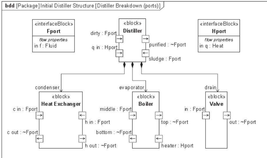
Figure 7. Distiller breakdown with ports.
