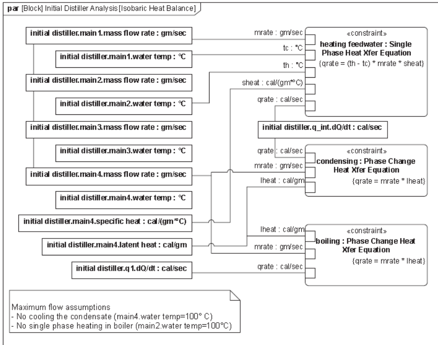
Figure 9. Defining parametric relationships as a prelude to analysis.
