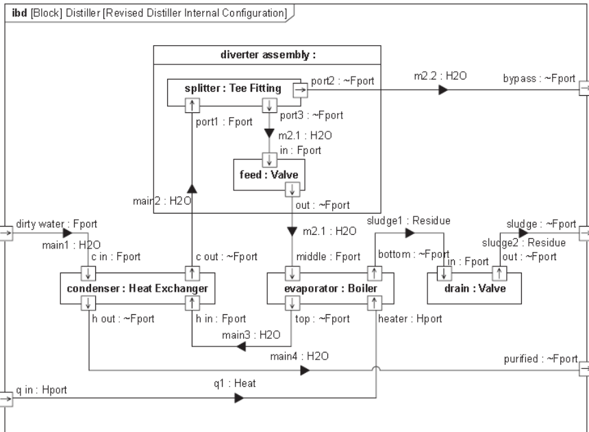
Figure 8. Internal block definition diagram depicting distiller configuration with item flow and allocation.
