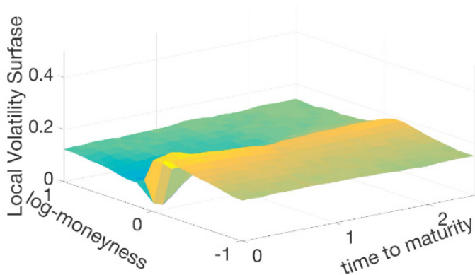
Figura 1: Local volatility surface estimated from EnKF-EnKF algorithm
