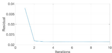
Figura 2: The left figure is the estimated spot prices and the right figure is the residual of every iteration.
